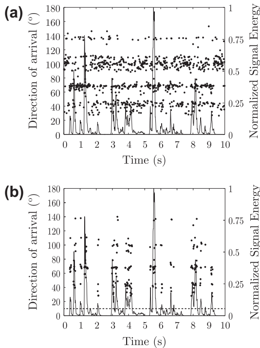
Fig. 5. (a) Estimated angles (dots) and normalized signal energy (line) for an analysis time of 10 s with the PHAT method in the office scenario. The sound is located at 60° and the SNR is 20 dB. (b) In this case the dots represent only those angles that will be accumulated in the histogram.
