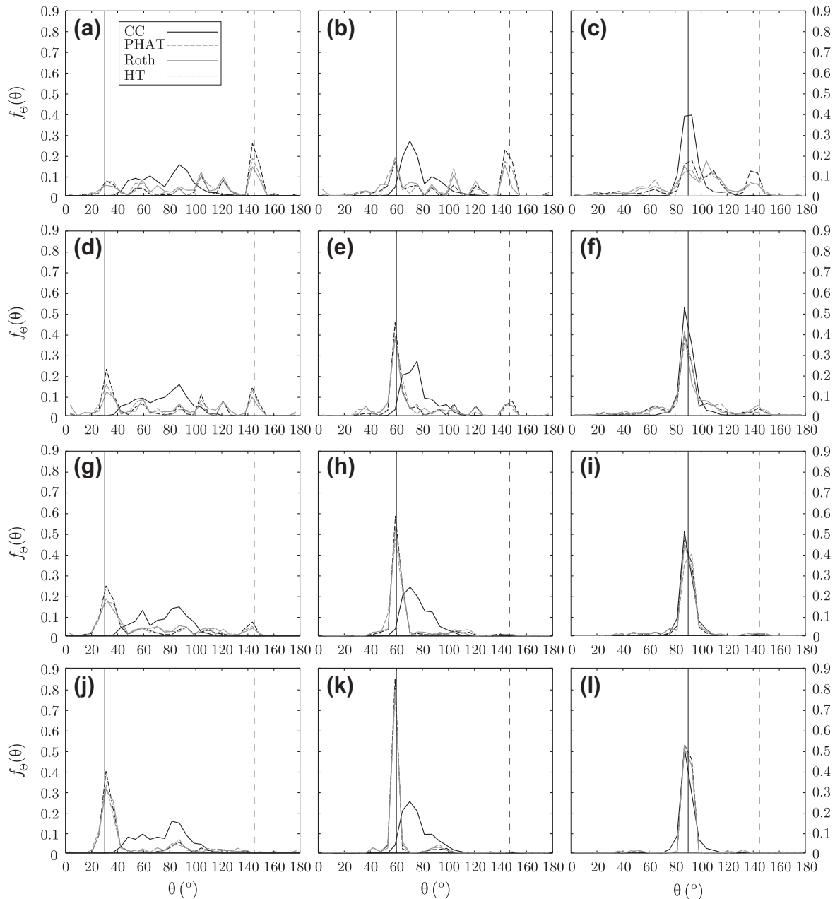
Fig. 6. Results obtained in lecture room scenario. Each subfigure contains the superimposed histograms of the four methods given a location of the source of sound and a signal-to-noise ratio. The signal-to-noise ratio is 10 dB from (a) to (c), 20 dB from (d) to (f), 30 dB from (g) to (i) and with ambient noise from (j) to (l). The source of sound (vertical line) is located at 30°, 60°, and 90° in the first, second and third column, respectively. The noise source (vertical dashed line) is located at 145°.
