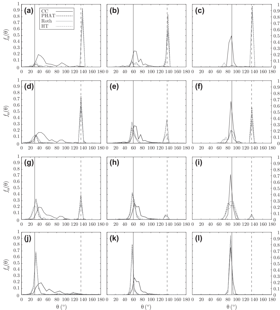
Fig. 9. Results obtained in auditorium scenario. Each subfigure contains the superimposed histograms of the four methods given a location of the source of sound and a signal-to-noise ratio. The signal-to-noise ratio is 10 dB from (a) to (c), 20 dB from (d) to (f), 30 dB from (g) to (i) and with ambient noise from (j) to (l). The source of sound (vertical line) is located at 30°, 60° and 90° in the first, second and third column, respectively. The noise source (vertical dashed line) is located at 135°.
