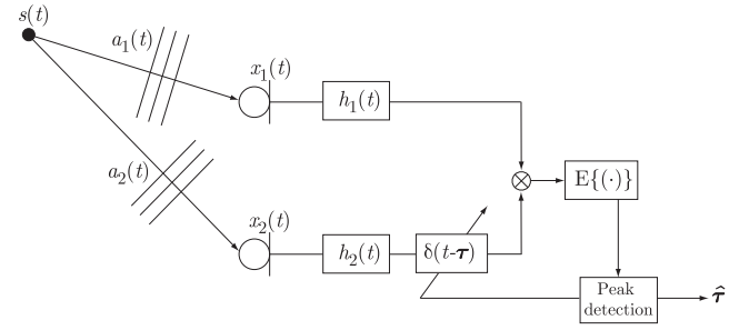
Fig. 1. Block diagram of a generalized cross-correlator for TDOA estimation [3].
