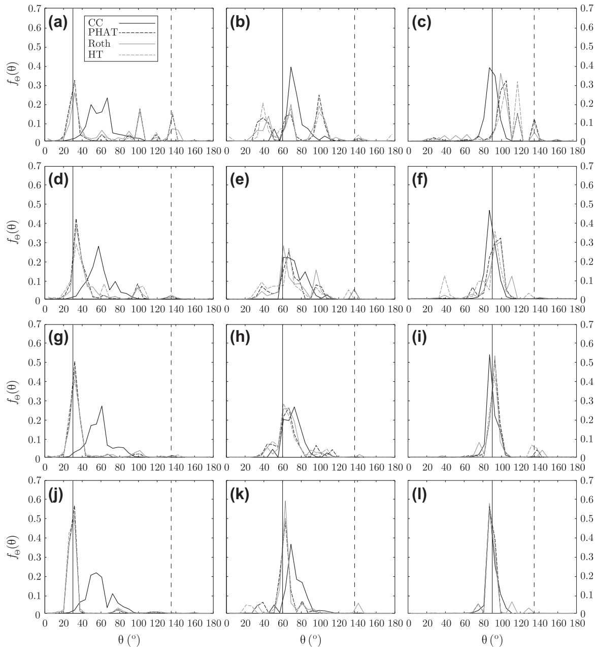
Fig. 7. Results obtained in office scenario. Each subfigure contains the superimposed histograms of the four methods given a location of the source of sound and a signal-to-noise ratio. The signal-to-noise ratio is 10 dB from (a) to (c), 20 dB from (d) to (f), 30 dB from (g) to (i) and with ambient noise from (j) to (l). The source of sound (vertical line) is located at 30°, 60° and 90° in the first, second and third column, respectively. The noise source (vertical dashed line) is located at 135°.
