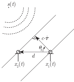
Fig. 4. Angle of incidence of a plane wave and \hat{\tau} . Angle \theta is the speaker location.
