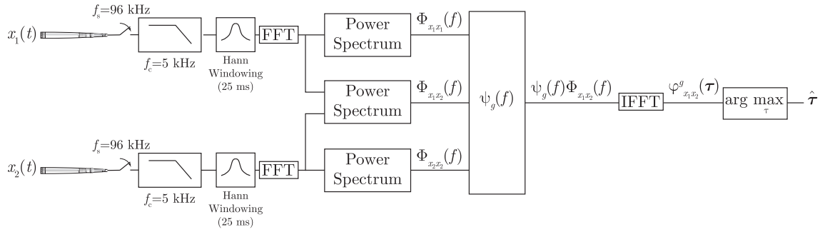
Fig. 3. Block diagram for the tested methods.
