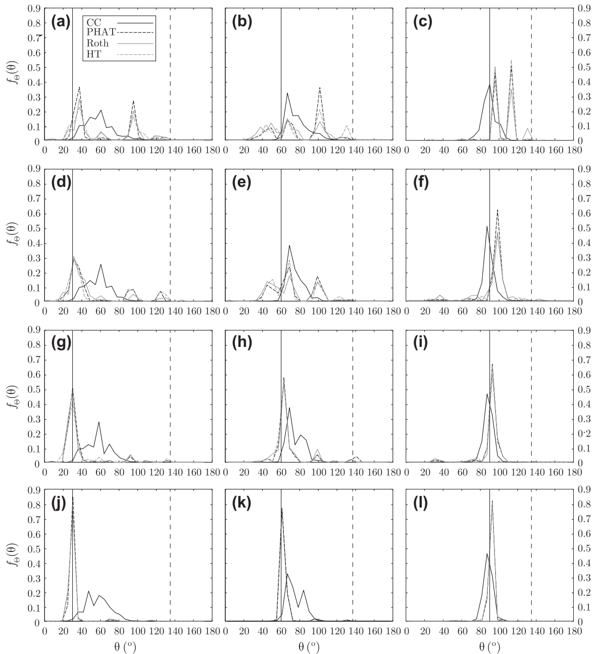
Fig. 8. Results obtained in modified office scenario. Each subfigure contains the superimposed histograms of the four methods given a location of the source of sound and a signal-to-noise ratio. The signal-to-noise ratio is 10 dB from (a) to (c), 20 dB from (d) to (f), 30 dB from (g) to (i) and with ambient noise from (j) to (l). The source of sound (vertical line) is located at 30°, 60° and 90° in the first, second and third column, respectively. The noise source (vertical dashed line) is located at 135°.
