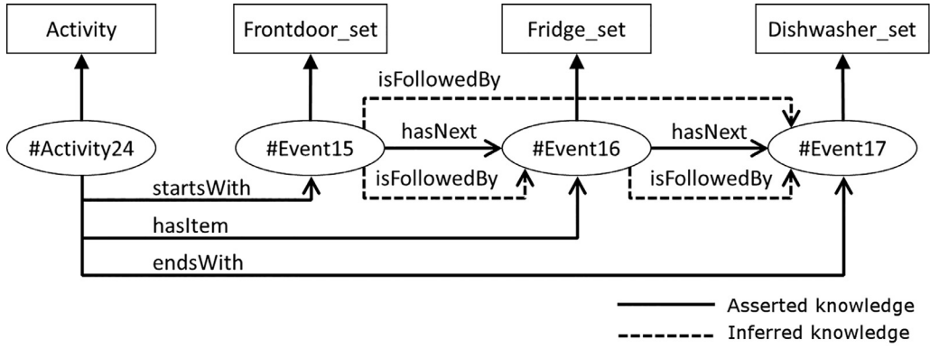
Fig. 2. Ontology example.
