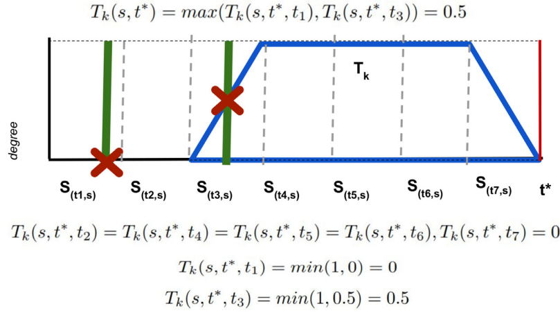
Fig. 3. Representation of a fuzzy temporal window T_k within a sensor activation in the segmented timeline S(s, t_i) . In the example, the aggregated degrees of activation T_k(s, t^*) are 0.5.
