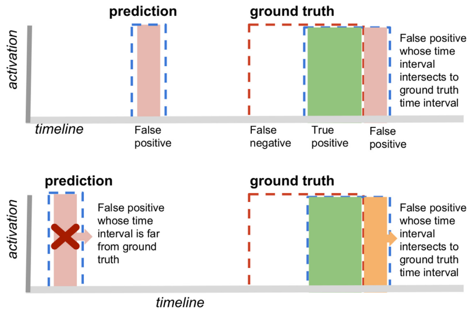
Fig. 5. Evaluation and metrics of predicted and ground truth activity time intervals in AR.
