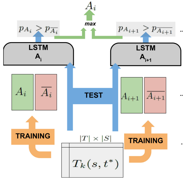
Fig. 4. Architecture of the ensemble of LSTM activity-based classifiers.
